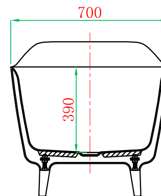
Section F-F
