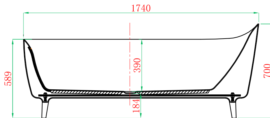
Section G-G
