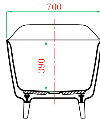
Section F-F
