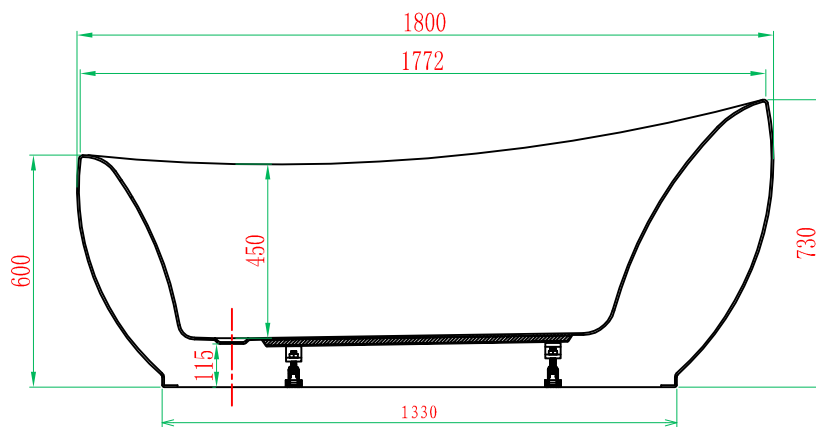
Section F-F
