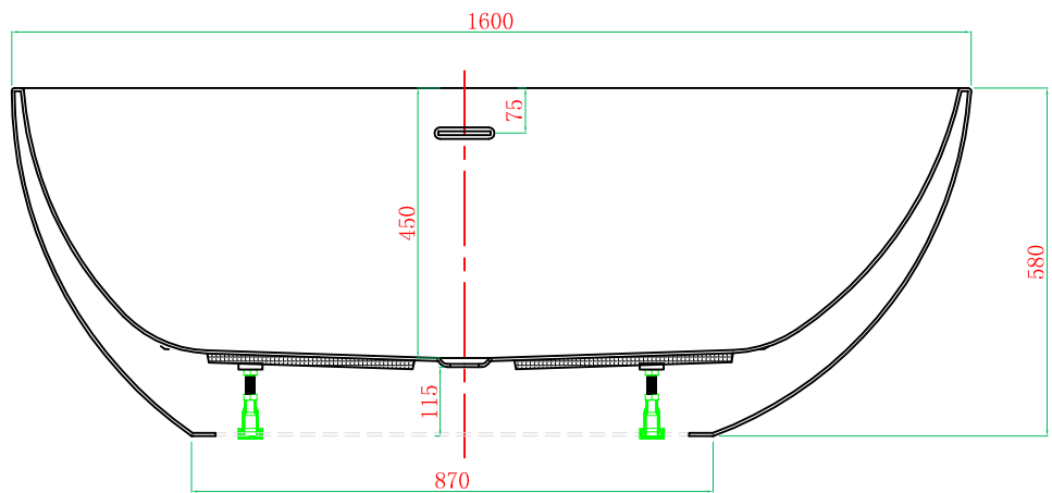
F-F
