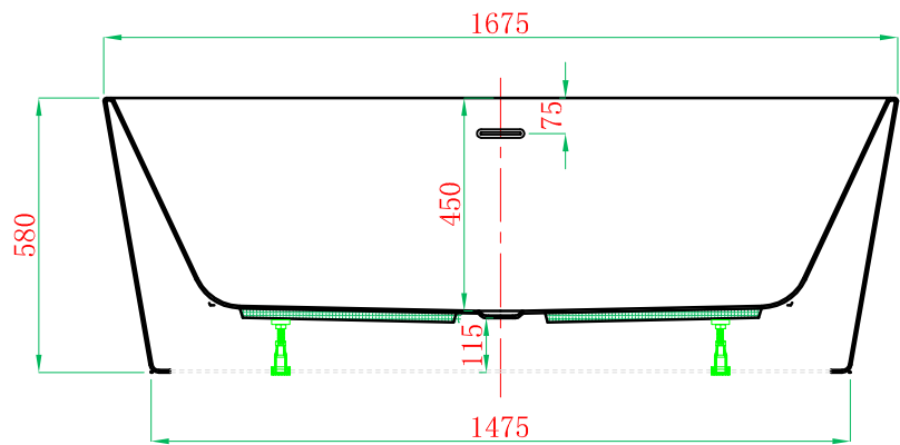
Cross Section F-F
