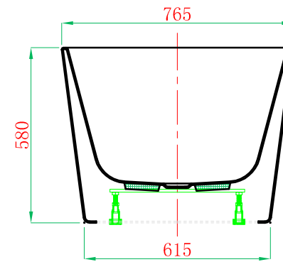
Cross Section G-G
