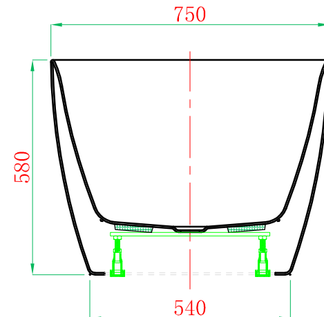
Cross Section G-G
